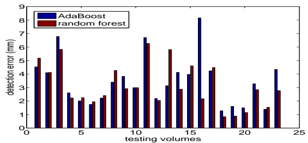
Fig. 5. Detection error of each testing CBCT volume
