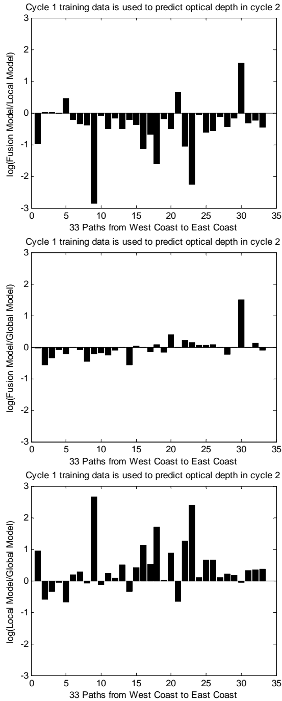
Figure 2 : Pairwise comparison of log MSE in E1. (a) Fusion model vs. Local Model ; (b) Fusion model vs. Global Model ; (c) Local model vs. Global model
