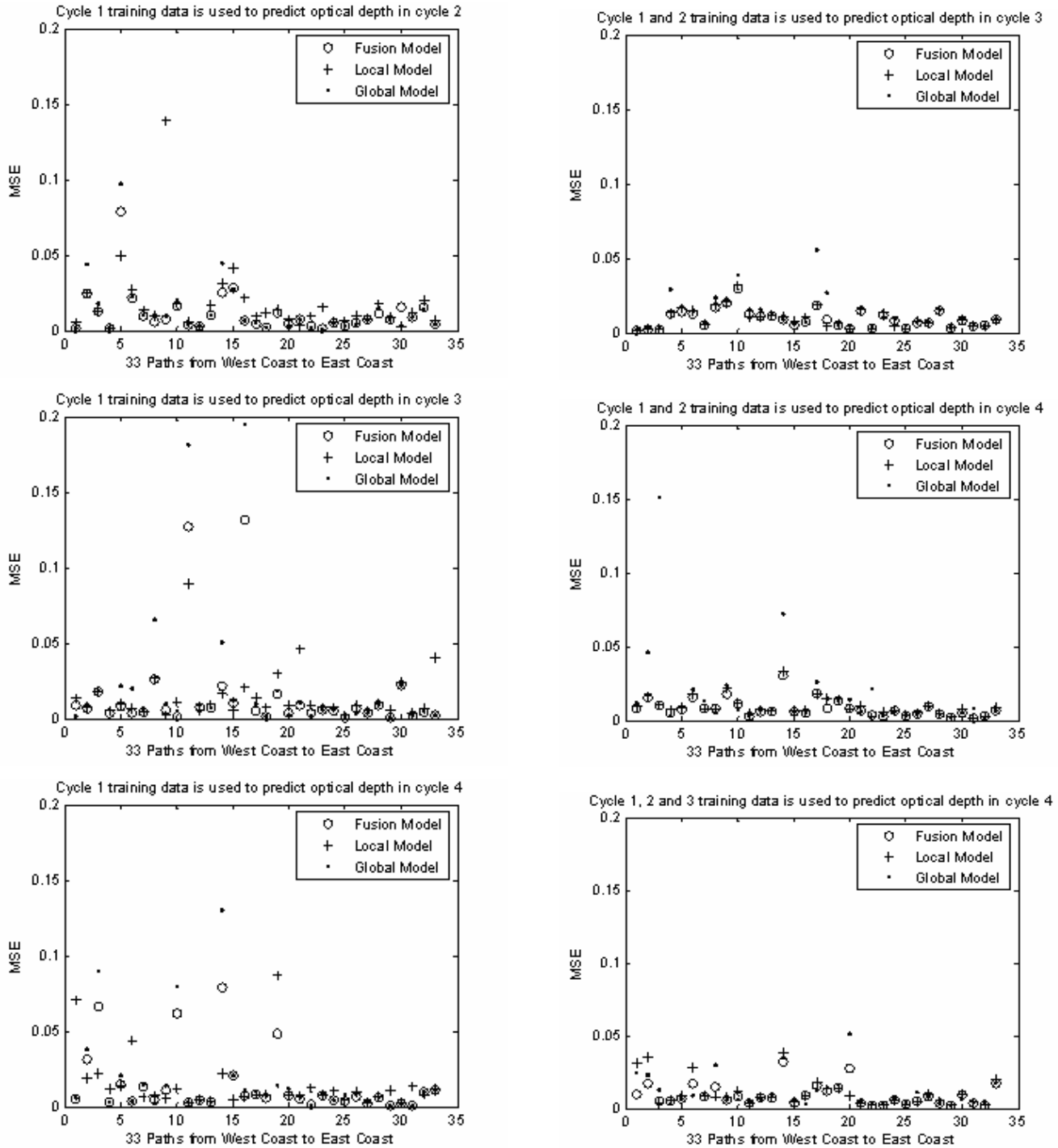
Figure 1: Comparison of MSE of three models on each path for E1 – E6 experiments
